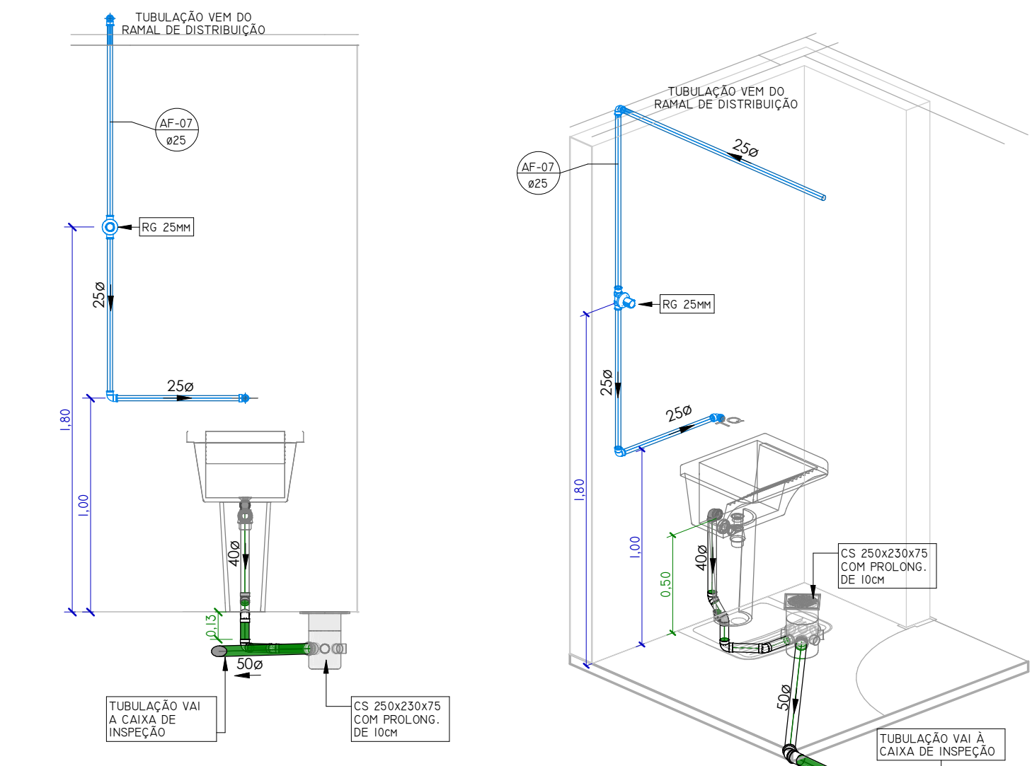
VISTA FRONTAL DML
