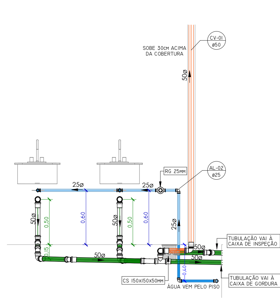
VISTA FRONTAL COPA
